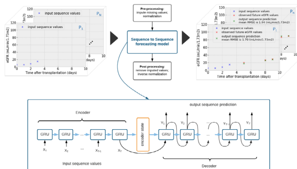
Figure 1. Schematic overview of the GRU Seq2Seq models for forecasting patient-specific kidney transplant function. The top panel shows the pipeline of the proposed model. The lower panel schematically illustrates the sequence-to-sequence model encoder-decoder architecture. First, N different patients' ( P_1 to P_N ) continuous eGFR values (input sequence values, X_1 – X_n , blue crosses) were pre-processed and then analyzed by the sequence-to-sequence model. The predictions from the model ( Y_1 – Y_n , green crosses) were post-processed and then evaluated by comparison with the observed eGFR values (red crosses) using the root mean square error (RMSE).
